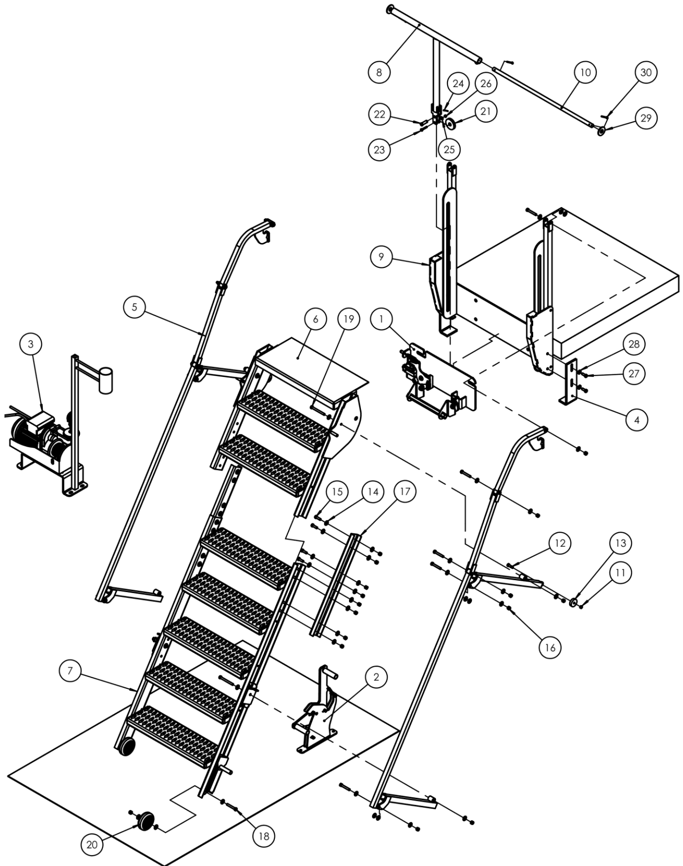
FIG. 2: LAD-FM-72 EXPLODED VIEW (44-006-711)
