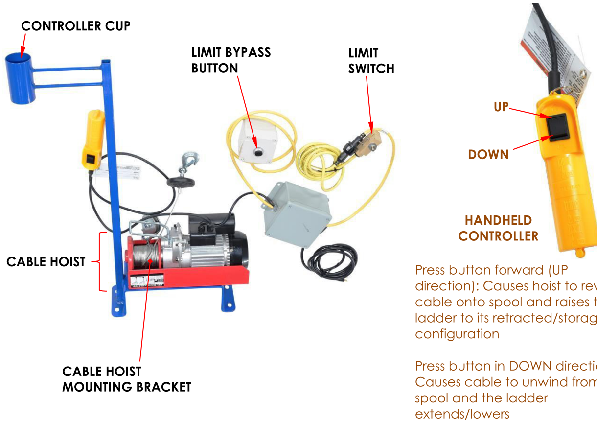
FIG. 7: CABLE HOIST, MOUNTING BRACKET, AND HANDHELD CONTROLLER
