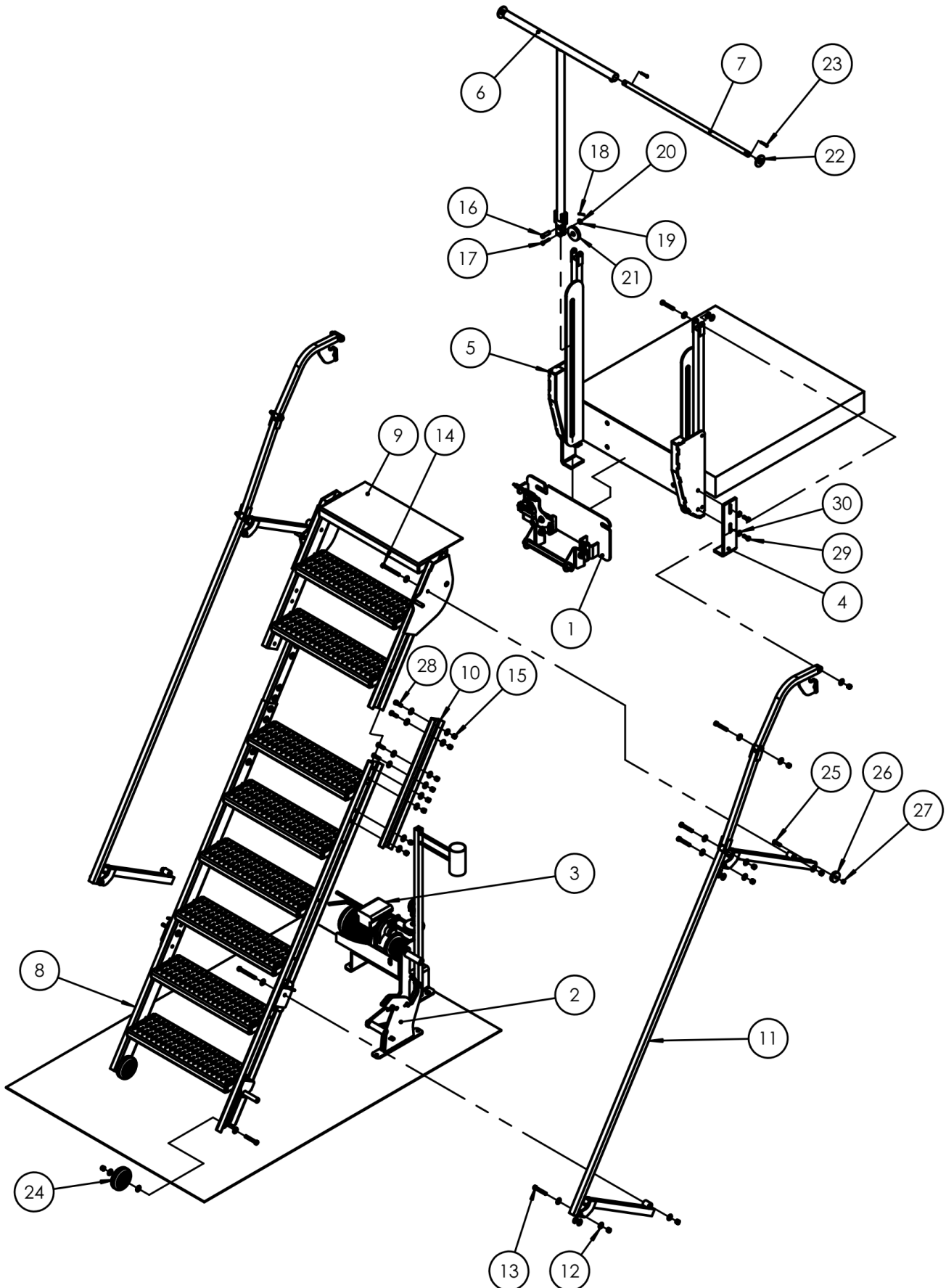
FIG. 3: LAD-FM-84 EXPLODED VIEW (44-006-712)
